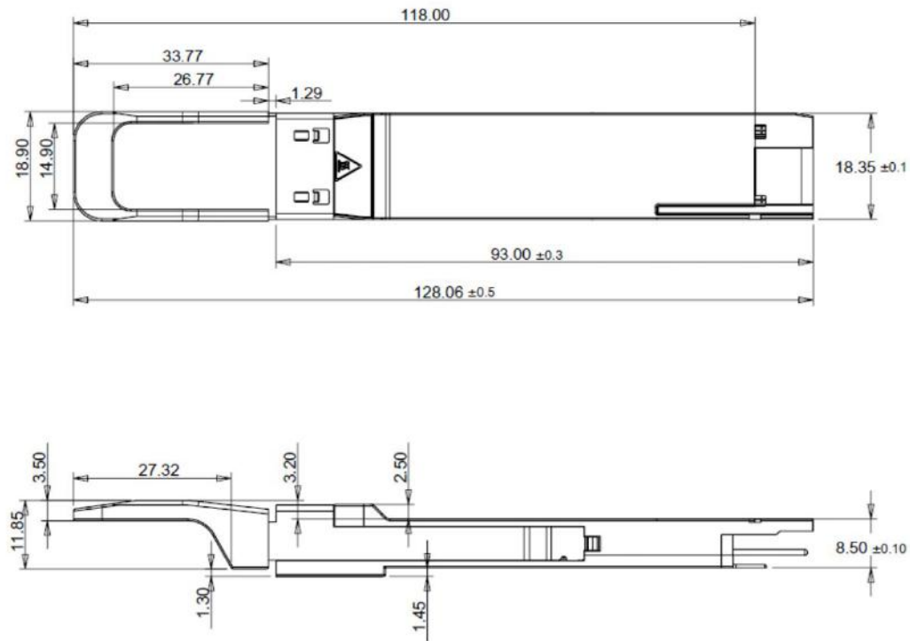
Figure 5. Mechanical Outline
