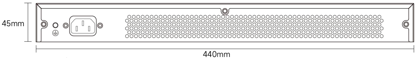
Back view
